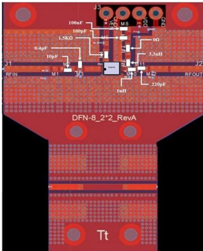
Figure 2.1 TL0375J-EVB-A 3300MHz ~ 3800MHz Schematic and EVB Layout
