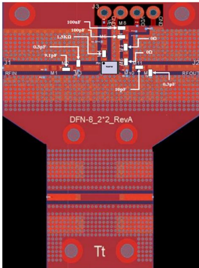
Figure 2.1 TL0375J-EVB-C 4400MHz ~ 5000MHz Schematic and EVB Layout
