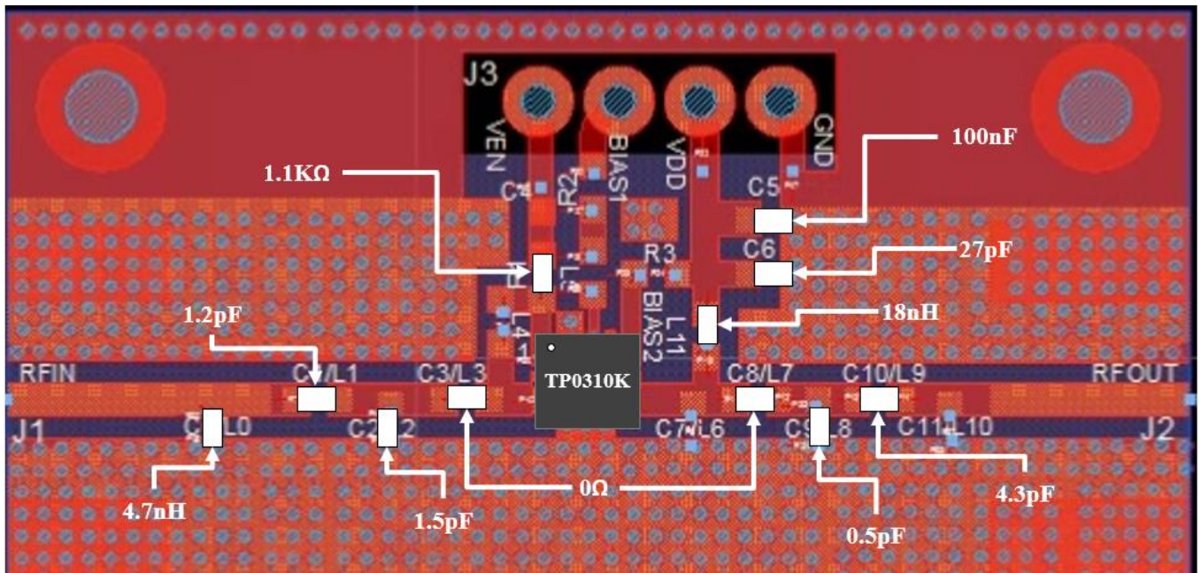
Figure 2.1 TP0310K-EVB-A 1700MHz ~ 2000MHz Schematic and EVB Layout
