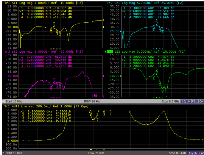
Figure 6.1.1. S parameters of TSL8029N-EVB-B RX-HG 5V 90mA
