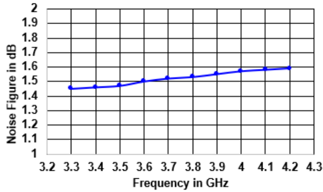
Figure 6.2.1. SMA-SMA Noise Figure of TSL8029N-EVB-B for 5V 90mA for RX-HG mode
