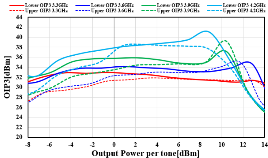
Figure 6.4.1 OIP3dBm vs P OUT /tone of TSL8029N-EVB-B for 5V 90mA for RX-HG mode
