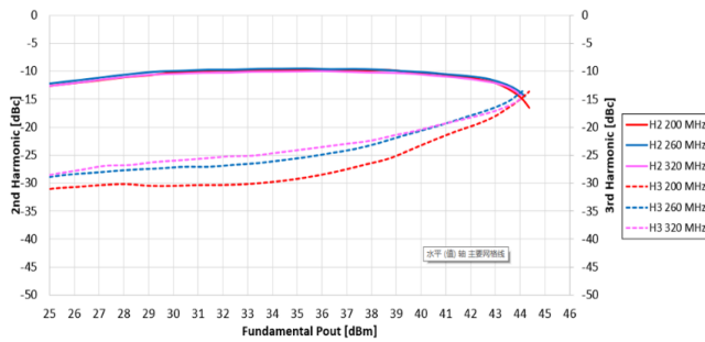
Figure 8.1.15 H2dBC and H3dBC v/s Pout TA9410E + TS8441L EVB-G, VD=50 V, IDQ=50 mA
