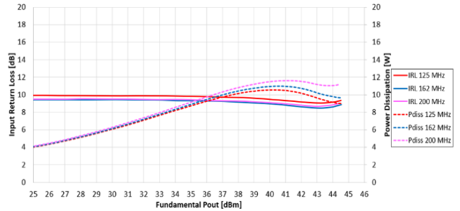
Figure 8.1.11 IRL and Pdis v/s Pout. Of TA9410E + TS8441L EVB-G, VD=50 V, IDQ=50 mA
