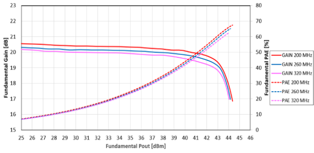
Figure 8.1.13 Gain, PAE v/s Pout Of TA9410E + TS8441L EVB-G, VD=50 V, IDQ= 50 mA
