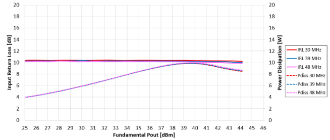
Figure 8.1.2 IRL and Pdis v/s Pout Of TA9410E + TS8441L EVB-G, VD=50 V, IDQ=50 mA
