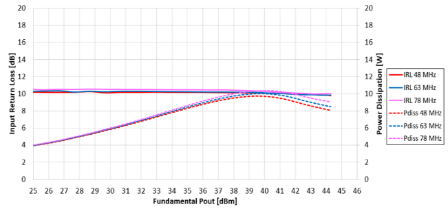
Figure 8.1.5 IRL and Pdiss v/s Pout Of TA9410E + TS8441L EVB-G, VD= 50 V, IDQ= 50 mA
