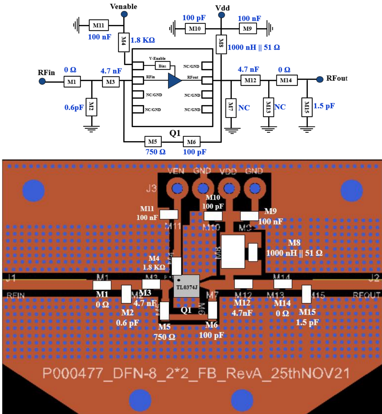
Figure 2.1 TL0374J-EVB-D1 30 MHz ~ 2600 MHz Schematic and EVB Layout
