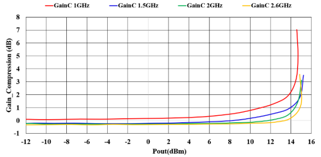
Figure 6.3.4. Gain compression Vs Pout of TL0374J-EVB-D1 [1-2.6 GHz]
