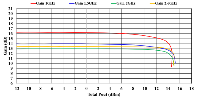
Figure 6.3.2. Gain Vs Pout of TL0374J-EVB-D1 [1-2.6GHz]
