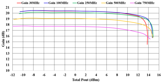
Figure 6.3.1. Gain Vs Pout of TL0374J-EVB-D1 [30-750 MHz]
