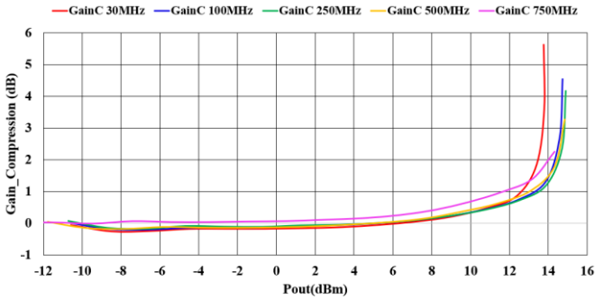
Figure 6.3.3. Gain compression Vs Pout of TL0374J-EVB-D1 [30-750 MHz]
