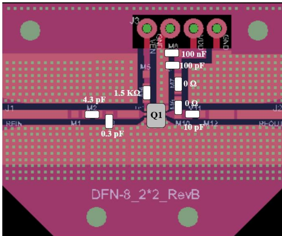
Figure 2.1 TL0375J-EVB-B 3700MHz ~ 4200MHz Schematic and EVB Layout
