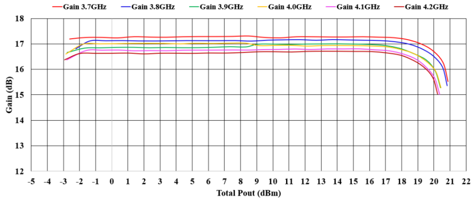
Figure 6.3.1. Gain Vs Pout of TL0375J-EVB-B
