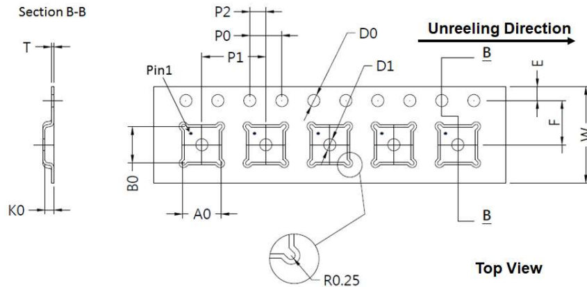
Figure 13 Tape and Reel Drawing
