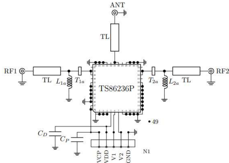
Figure 5b. 10 MHz – 1000 MHz circuit schematic.
