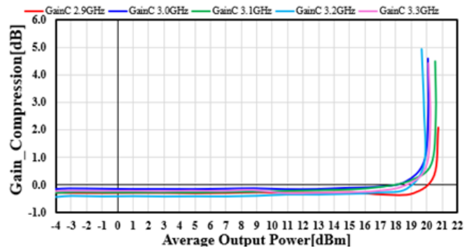
Figure 6.3.4 Gain compression vs P_{OUT} of TSL8029N-EVB-E for 5 V, 90 mA for RX-HG mode
