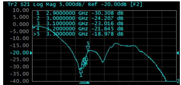
Figure 6.1.5. ANT to TX isolation of TSL8029N-EVB-E when RX-HG is on
