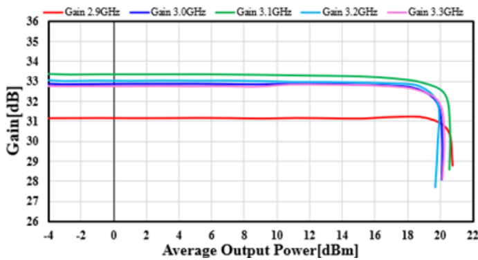
Figure 6.3.3. Gain vs P_{OUT} of TSL8029N-EVB-E for 5 V, 90 mA for RX-HG mode
